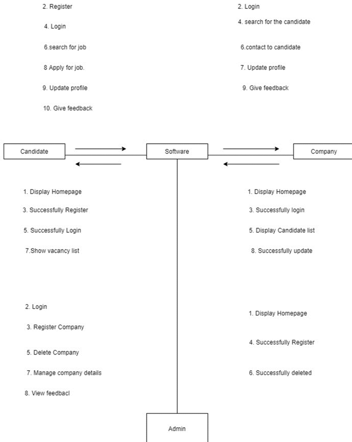
Fig 6.9 Collaboration Diagram
