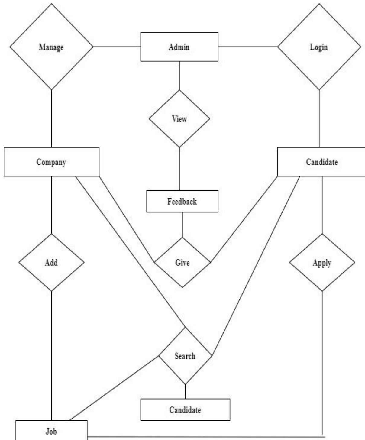
Fig 6.1: E-R Diagram
