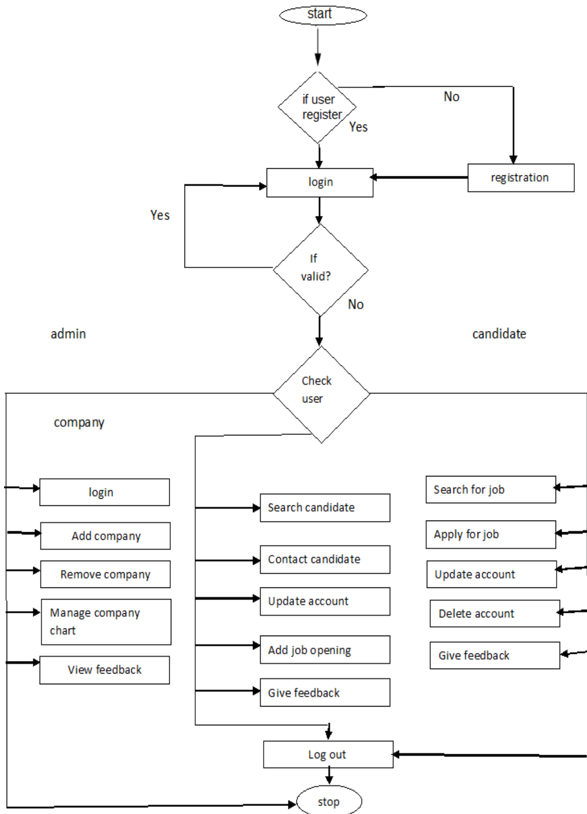
Fig. 6.4: Activity Diagram
